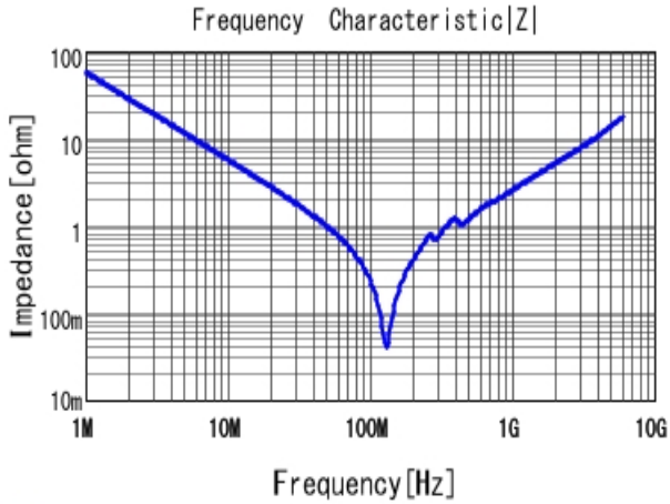
■ GRM1885C1H272JA01 |Z| DCOV, 25degC
