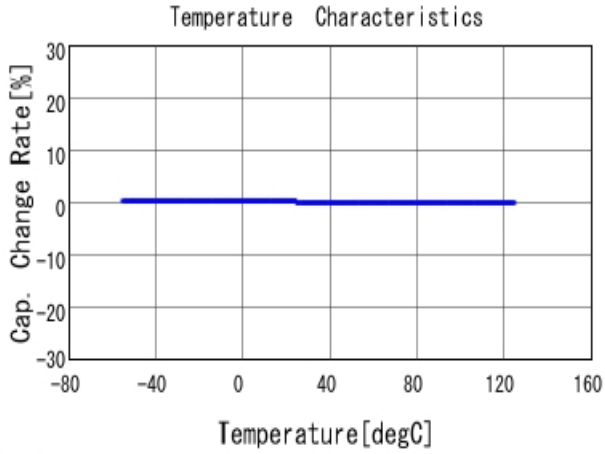
■ GRM1885C1H272JA01 C-Temp. capchange, DCOV, AC1Vrms
