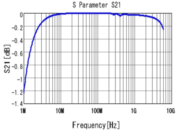
■ GRM1885C1H272JA01 S21 DCOV, 25degC
