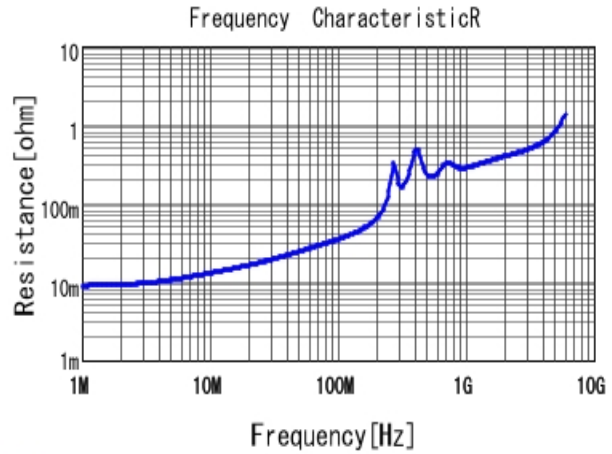
■ GRM1885C1H272JA01 R DCOV, 25degC
