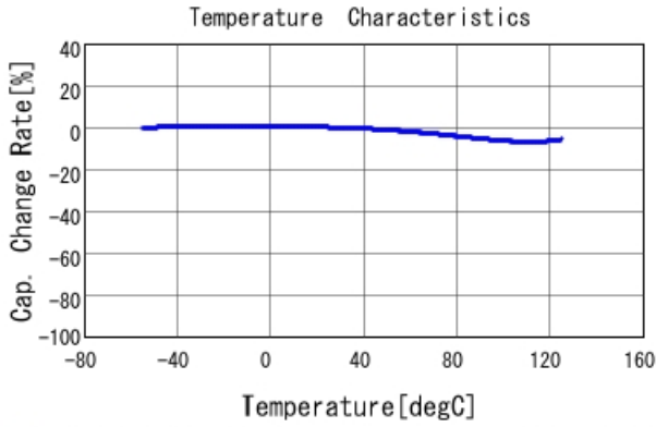
■ GRM033R71C102KA01 C-Temp. capchange, DCO. 0V, AC1. 0Vrm
