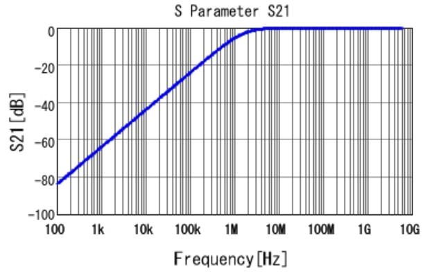
■ GRM033R71C102KA01 S21 DCOV, 25degC
