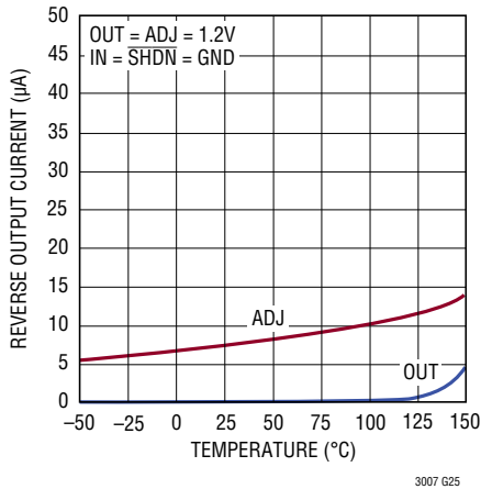
Reverse-Output Current
