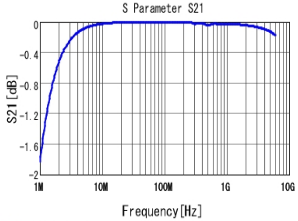
■ GRM1885C1H222JA01 S21 DCOV, 25degC
