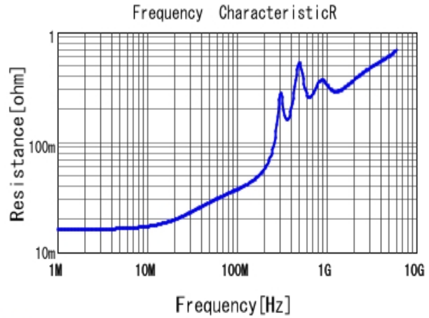
■ GRM1885C1H222JA01 R DCOV, 25degC
