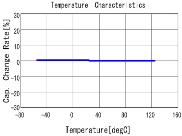
■ GRM1885C1H222JA01 C-Temp. capchange, DCOV, AC1Vrms
