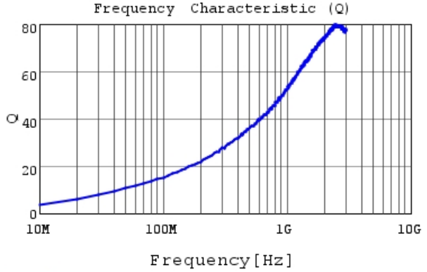
LQG15WZ3N6B02 Q
