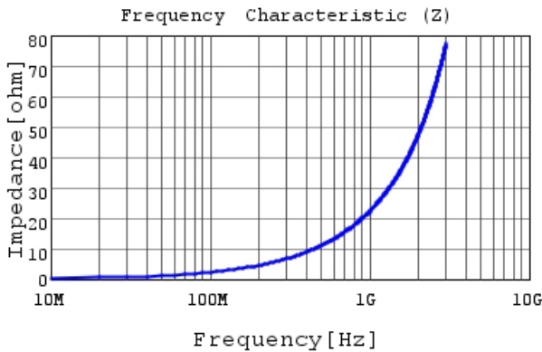
LQG15WZ3N6B02 |Z|
