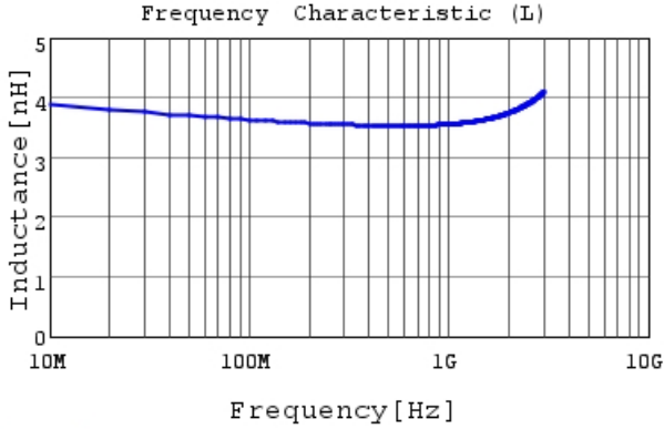
LQG15WZ3N6B02 L
