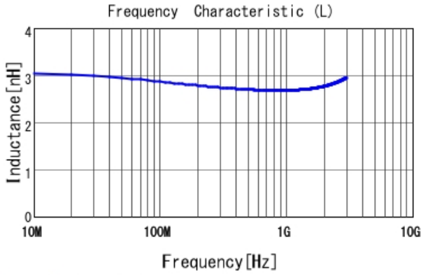
LQP03TG2N7B02 L
