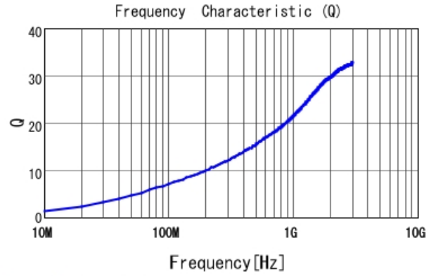
LQP03TG2N7B02 Q
