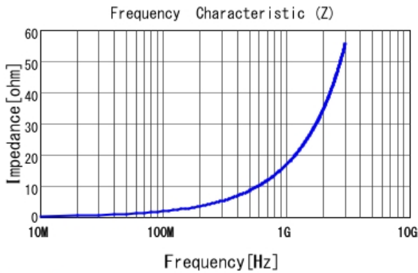
LQP03TG2N7B02 |Z|
