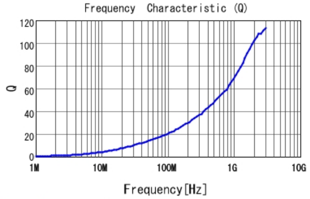
LQW15AN2N9B8Z Q
