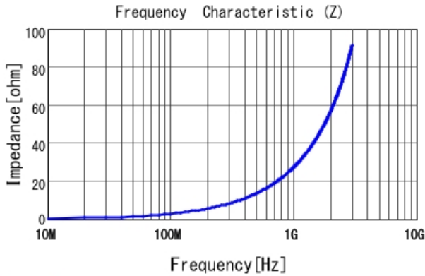
LQP03TQ4N3J02 |Z|
