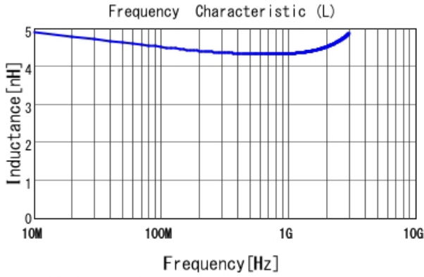
LQP03TQ4N3J02 L
