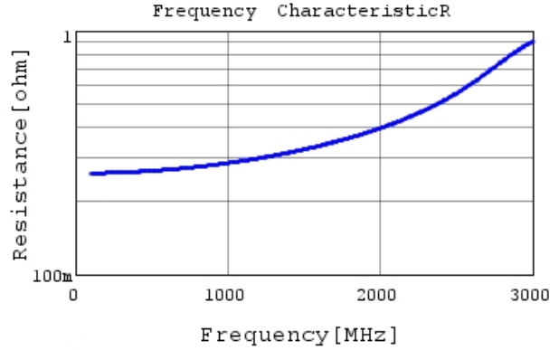
GRM31A5C2J100GW01 R DCOV, 25degC
