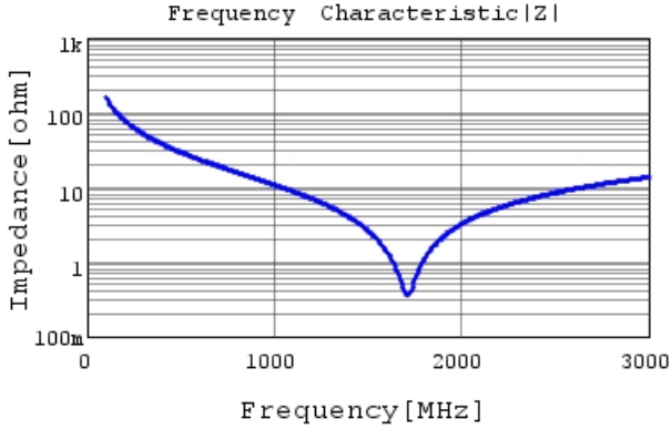
GRM31A5C2J100GW01 |Z| DCOV, 25degC
