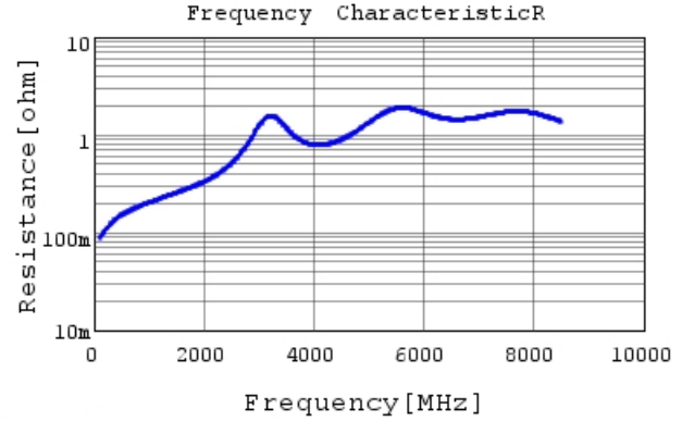
GCM1555C1H330JA16 R DC0V, 25degC
