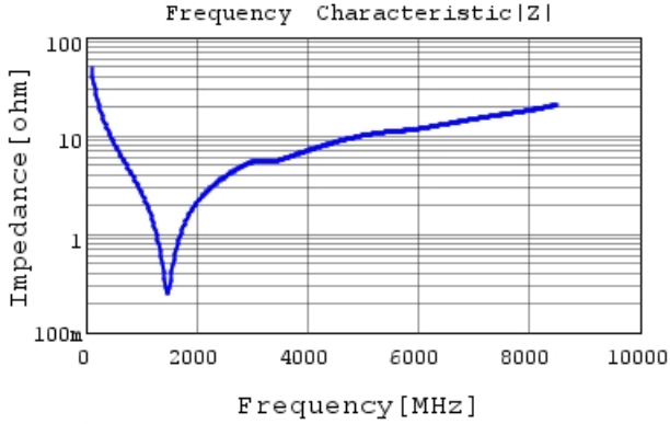
GCM1555C1H330JA16 |Z| DC0V, 25degC
