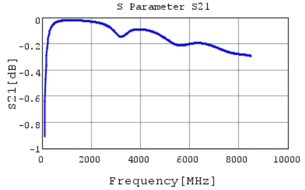
GCM1555C1H330JA16 S21 DCOV, 25degC
