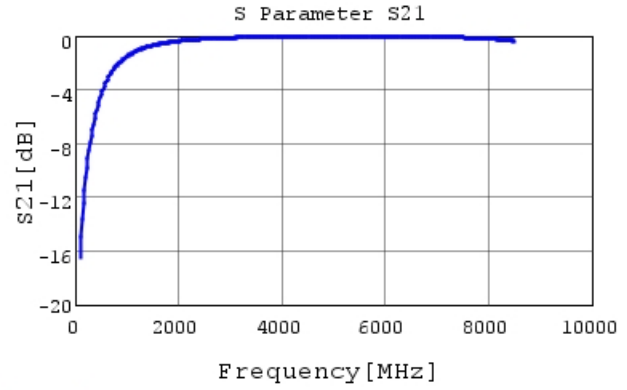
GCQ1555C1H2R4WB01 S21 DCOV, 25degC
