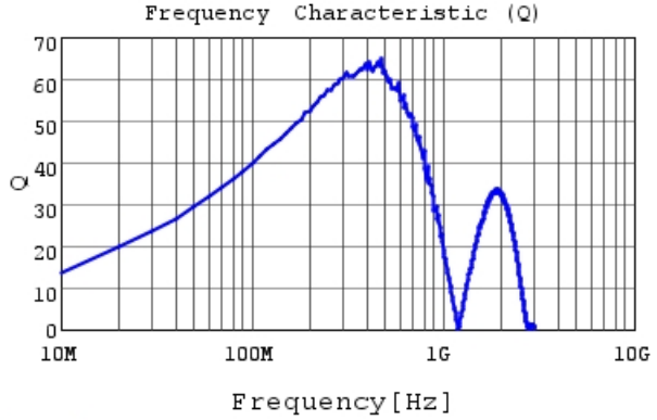
LQW2BASR12J00 Q
