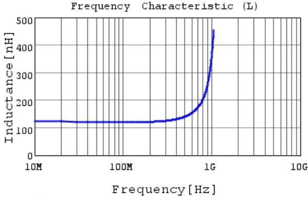
LQW2BASR12J00 L
