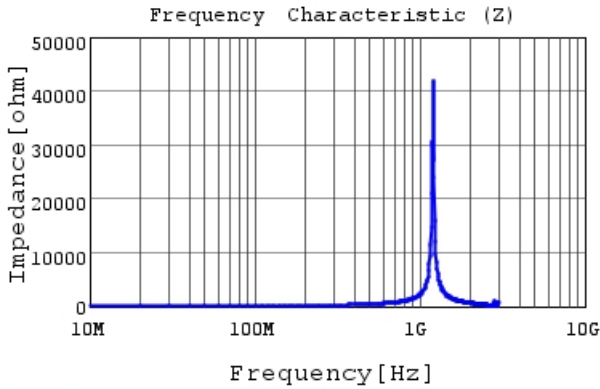
LQW2BASR12J00 |Z|
