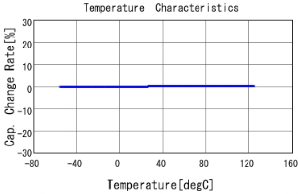
GRM21A5C2E100JW01 C-Temp. capchange, DC0V, AC1Vrms
