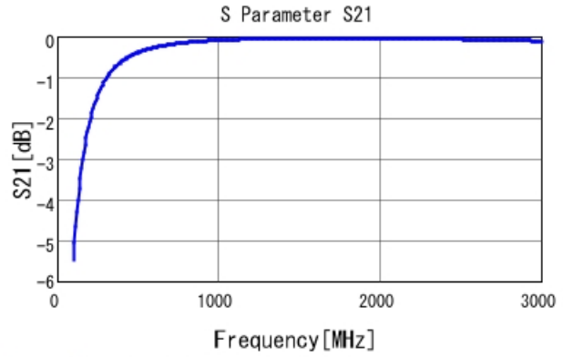
GRM21A5C2E100JW01 S21 DC0V, 25degC
