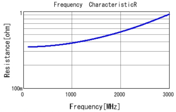
GRM21A5C2E100JW01 R DCOV, 25degC
