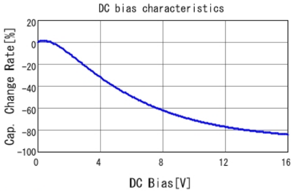
GRM32ER61C476ME15 C-DC bias capchange, 25.0degC, A
