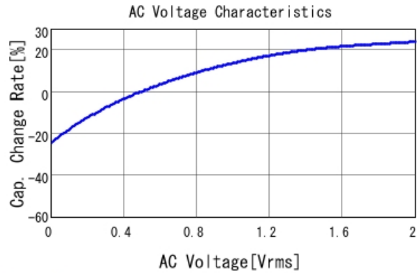
GRM32ER61C476ME15 C-AC Voltage capchange, DCOV, 25
