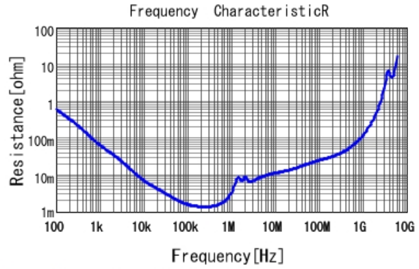
GRM32ER61C476ME15 R DCOV, 25degC
