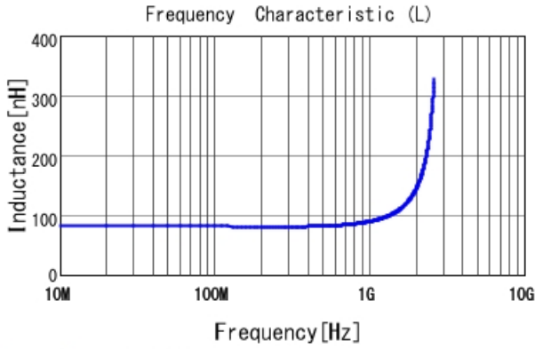
LQW15AN82NG0Z L
