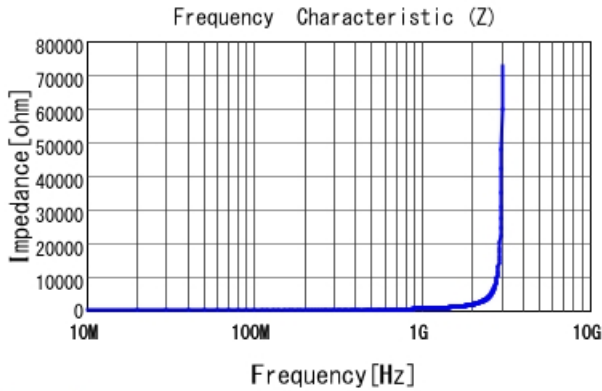
LQW15AN82NG0Z |Z|
