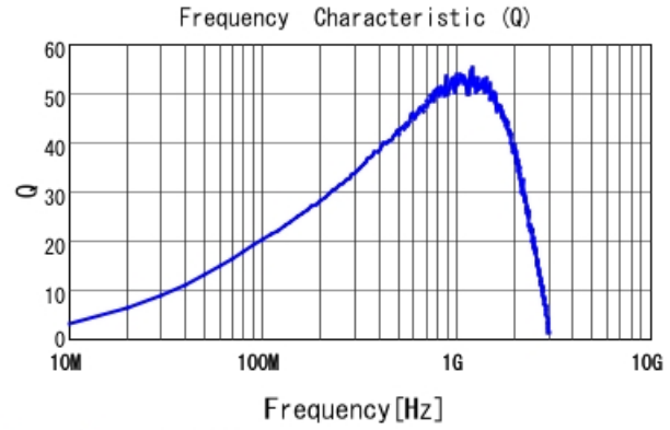
LQW15AN82NG0Z Q
