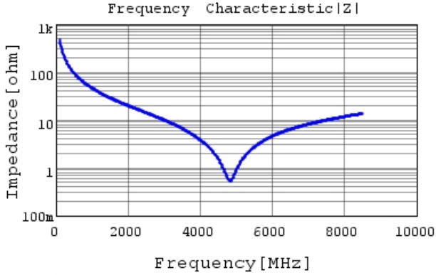
GCM1555C1H3R3BA16 |Z| DC0V, 25degC
