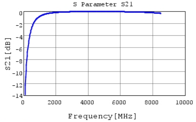
GCM1555C1H3R3BA16 S21 DCOV, 25degC
