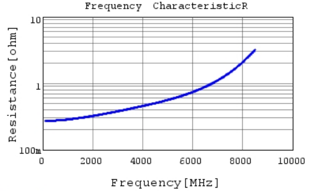
GCM1555C1H3R3BA16 R DC0V, 25degC
