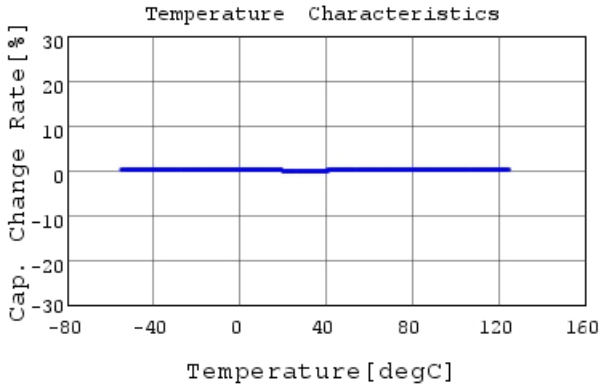
GCM1555C1H3R3BA16 C-Temp. capchange, DCOV, 1
