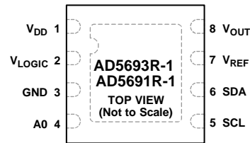
Figure 7. AD5693R-1/AD5691R-1 Pin Configuration, 8-Lead LFCSP, V_{\text{LOGIC}} Option
