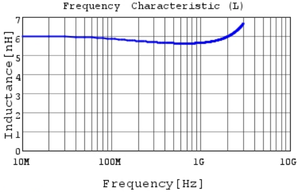
LQP15MN5N6B02 L
