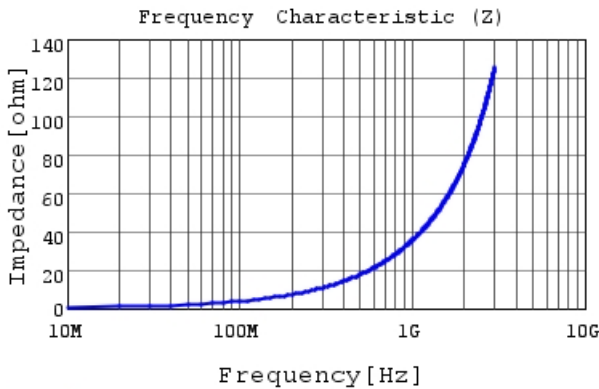
LQP15MN5N6B02 |Z|
