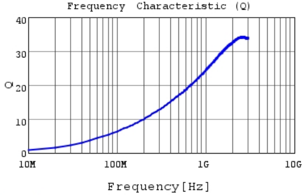
LQP15MN5N6B02 Q
