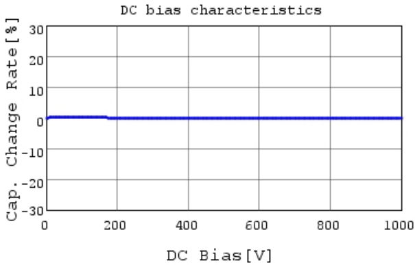
GRM31C5C3A821FWA3 C-DC bias capchange, 25.0c
