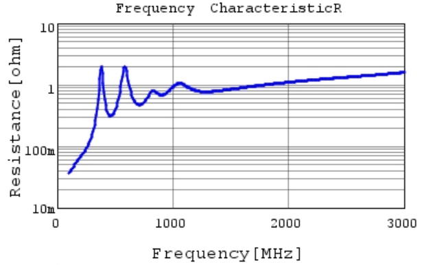
GRM31C5C3A821FWA3 R DC0V, 25degC
