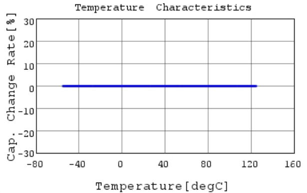
GRM31C5C3A821FWA3 C-Temp. capchange, DC0V, 1
