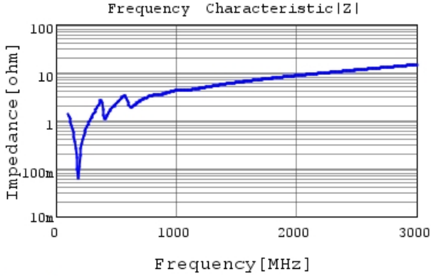
GRM31C5C3A821FWA3 |Z| DC0V, 25degC
