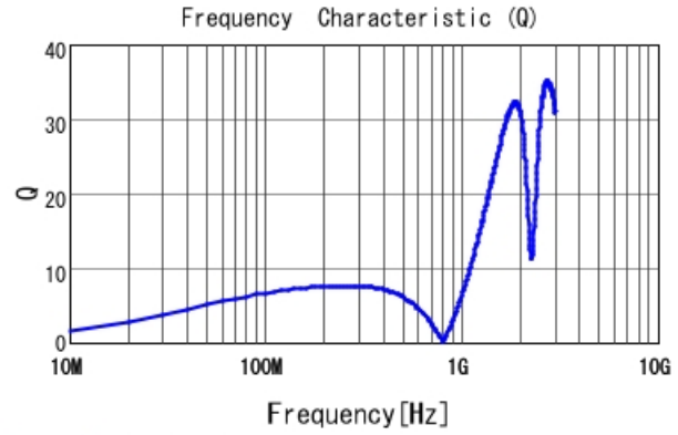
LQP03TNR16J02 Q
