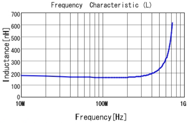
LQP03TNR16J02 L
