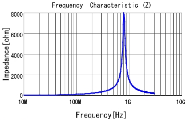
LQP03TNR16J02 |Z|
