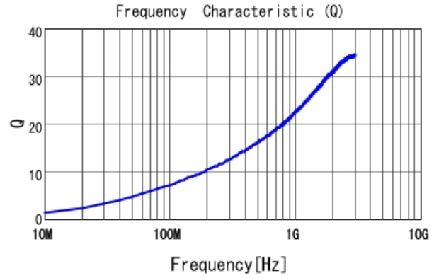
LQP03TG2N8B02 Q
