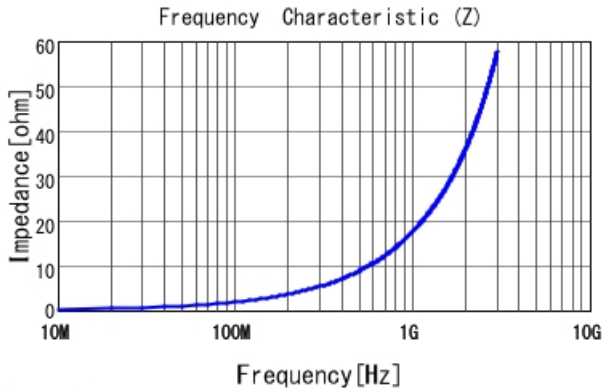
LQP03TG2N8B02 |Z|
