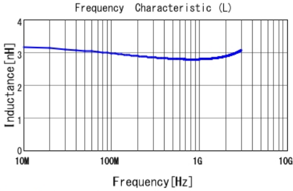
LQP03TG2N8B02 L
