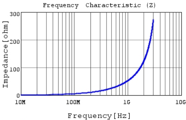
LQG18HN8N2J00 |Z|
