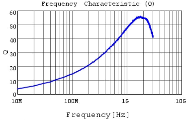
LQG18HN8N2J00 Q
