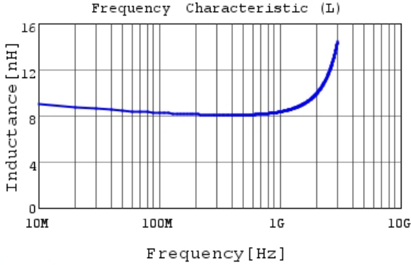
LQG18HN8N2J00 L
