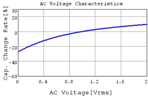
GRM21BZ71H475ME15 C-AC Voltage capchange, Dc
