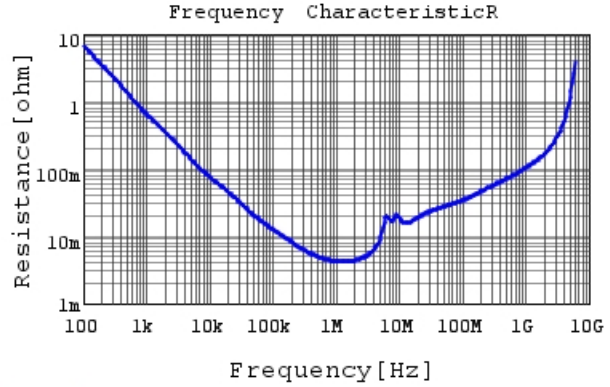
GRM21BZ71H475ME15 R DCOV, 25degC
