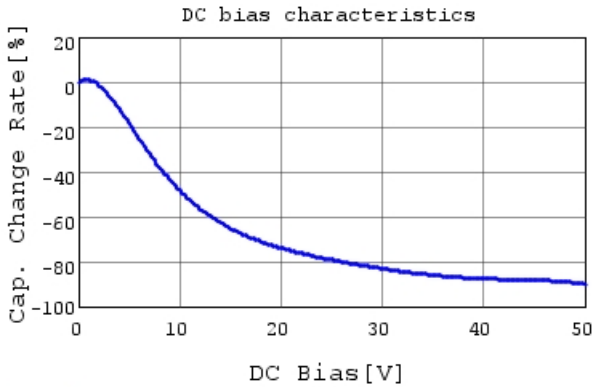
GRM21BZ71H475ME15 C-DC bias capchange, 25.0c
