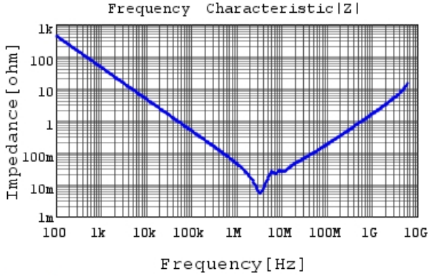
GRM21BZ71H475ME15 |Z| DCOV, 25degC
