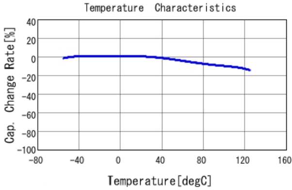
GCJ188R71C224KA01 C-Temp. capchange, DC0.0V, AC1.C
