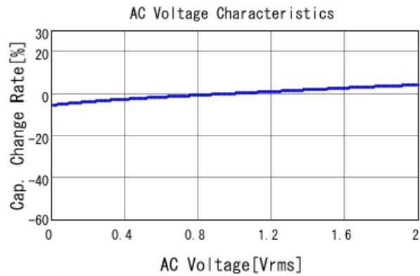
GCJ188R71C224KA01 C-AC Voltage capchange, DCOV, 25
