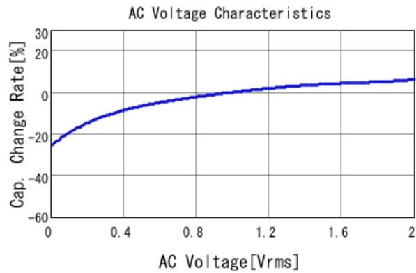
GCM155C71A474KE36 C-AC Voltage capchange, DCOV, 25
