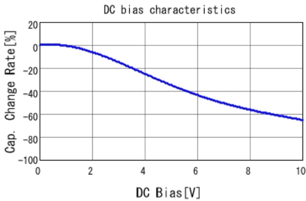
GCM155C71A474KE36 C-DC bias capchange, 25.0degC, A
