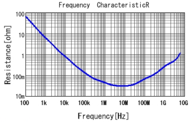
GCM155C71A474KE36 R DCOV, 25degC
