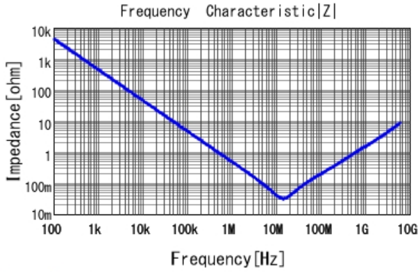
GCM155C71A474KE36 |Z| DCOV, 25degC
