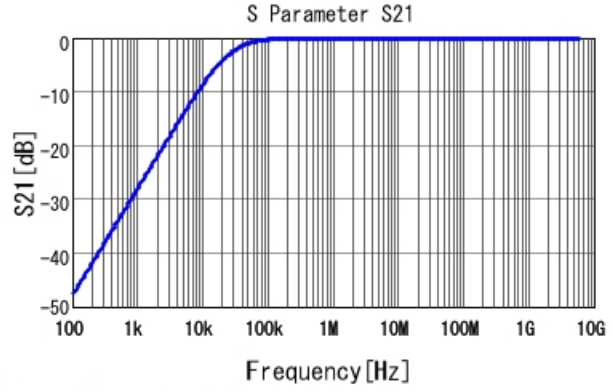
GRM155R61A683KA01 S21 DC0V, 25degC
