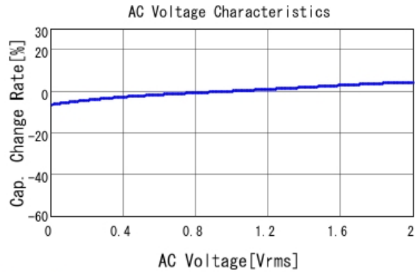
GRM155R61A683KA01 C-AC Voltage capchange, DCOV, 25
