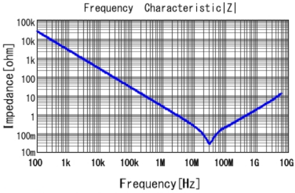
GRM155R61A683KA01 |Z| DCOV, 25degC
