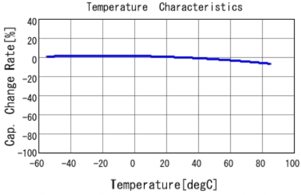
GRM155R61A683KA01 C-Temp. capchange, DC0.0V, AC1.C
