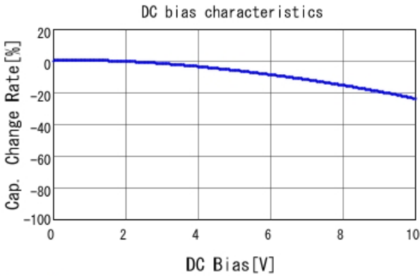
GRM155R61A683KA01 C-DC bias capchange, 25.0degC, A
