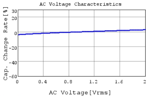
GCM21BR71H105KA03 C-AC Voltage capchange, Dc
