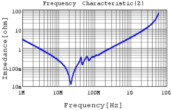
GRM31C5C2A563JA01 |Z| DC0V, 25degC
