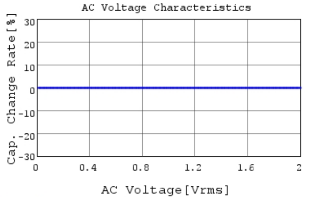
GRM31C5C2A563JA01 C-AC Voltage capchange, DC
