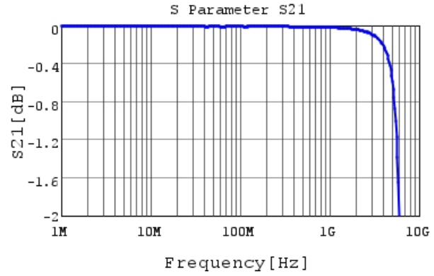
GRM31C5C2A563JA01 S21 DCOV, 25degC
