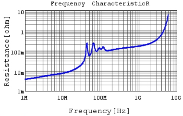
GRM31C5C2A563JA01 R DC0V, 25degC
