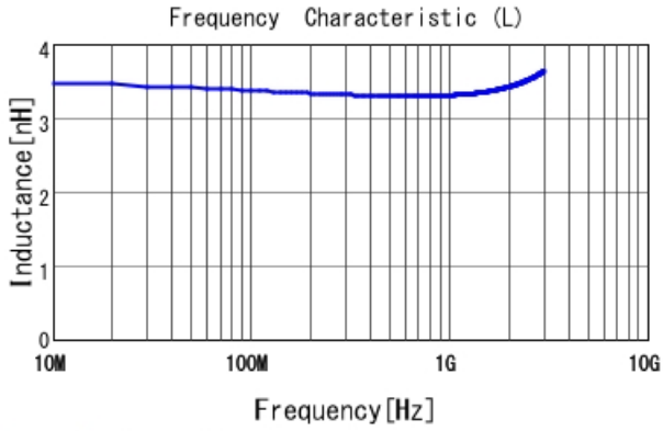
LQP03HQ3N3C02 L
