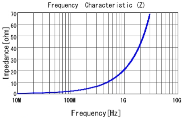
LQP03HQ3N3C02 |Z|
