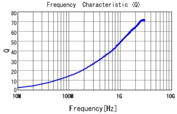
LQP03HQ3N3C02 Q
