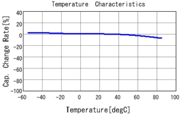
GRM155R61E222KA01 C-Temp. capchange, DC0.0V, AC1.C
