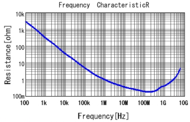
GRM155R61E222KA01 R DCOV, 25degC
