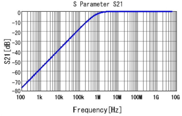
GRM155R61E222KA01 S21 DC0V, 25degC
