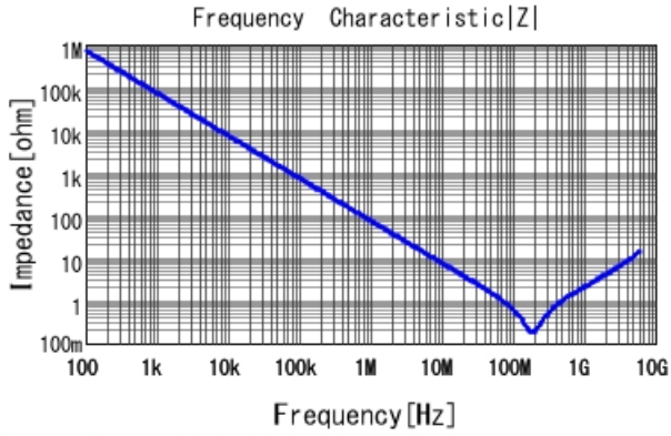
GRM155R61E222KA01 |Z| DCOV, 25degC
