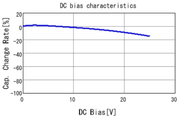
GRM155R61E222KA01 C-DC bias capchange, 25.0degC, A
