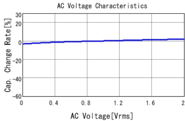
GRM155R61E222KA01 C-AC Voltage capchange, DCOV, 25
