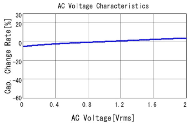
GRM319R61A105KA01 C-AC Voltage capchange, DCOV, 25
