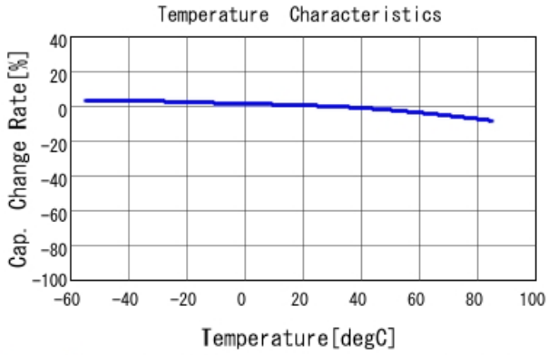
GRM319R61A105KA01 C-Temp. capchange, DC0.0V, AC1.C
