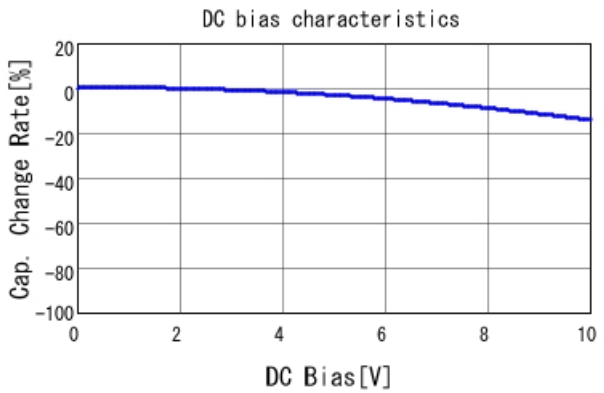
GRM319R61A105KA01 C-DC bias capchange, 25.0degC, A
