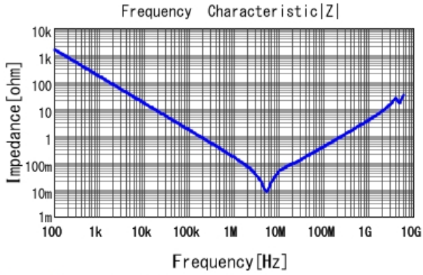
GRM319R61A105KA01 |Z| DCOV, 25degC
