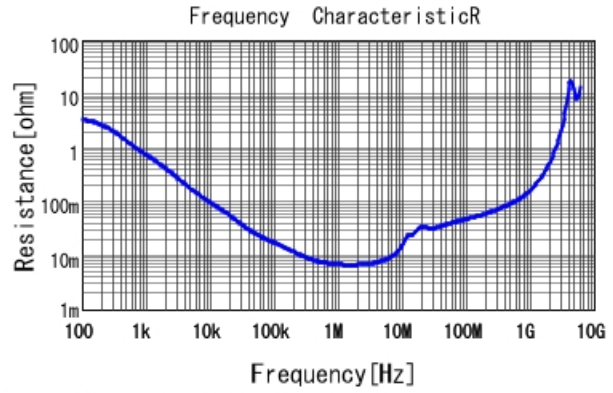
GRM319R61A105KA01 R DCOV, 25degC
