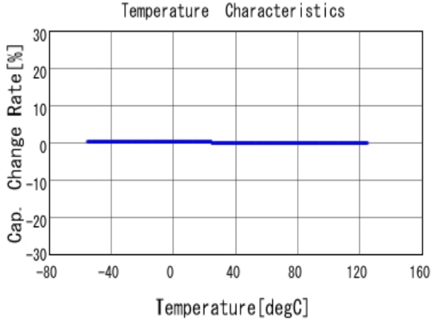
■ GRM2165C1H182JA01 C-Temp. capchange, DCOV, AC1Vrms
