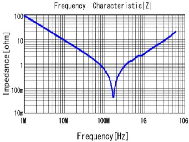
■ GRM2165C1H182JA01 |Z| DCOV, 25degC
