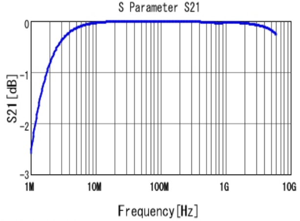
■ GRM2165C1H182JA01 S21 DCOV, 25degC
