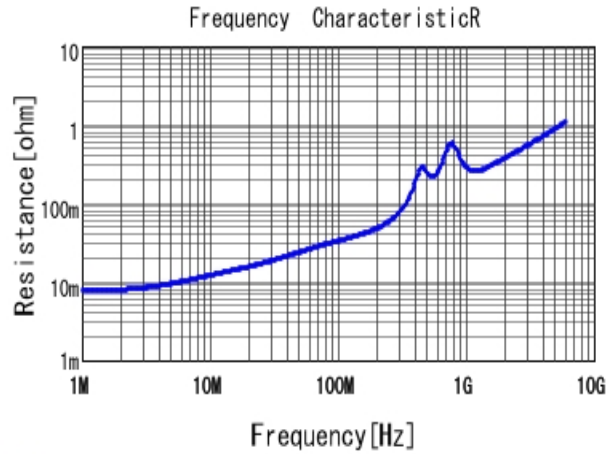
■ GRM2165C1H182JA01 R DCOV, 25degC
