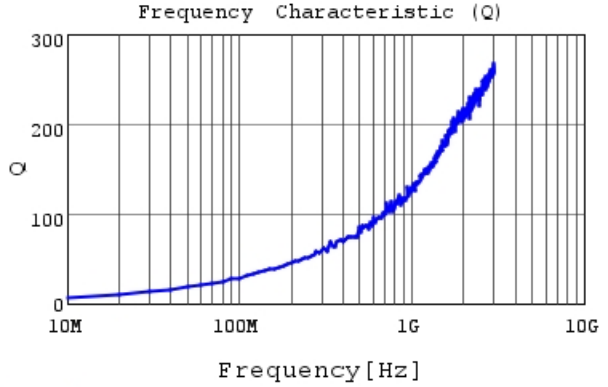
LQG18HN1N2S00 Q
