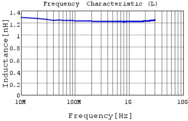
LQG18HN1N2S00 L
