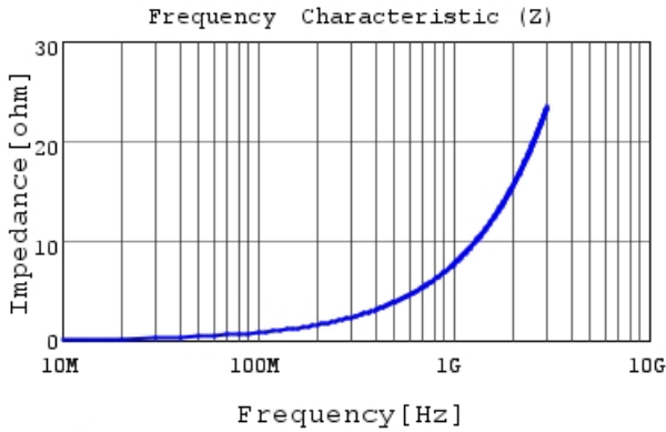
LQG18HN1N2S00 |Z|
