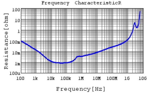
GRM32ER60G337ME05 R DCOV, 25degC
