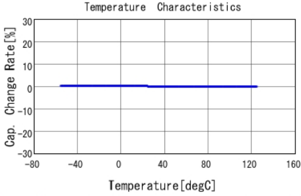
GRM0335C1E5R6BA01 C-Temp. capchange, DC0V, AC1Vrms
