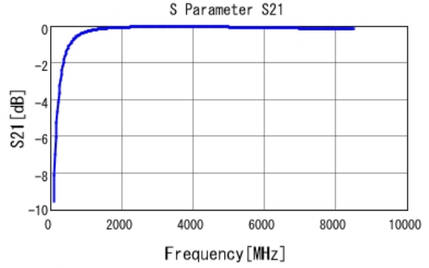
GRM0335C1E5R6BA01 S21 DC0V, 25degC
