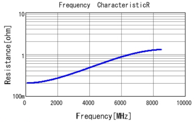
GRM0335C1E5R6BA01 R DCOV, 25degC
