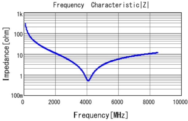
GRM0335C1E5R6BA01 |Z| DCOV, 25degC
