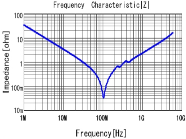
■ GRM2162C1H472JA01 |Z| DCOV, 20degC
