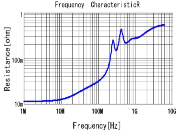
■ GRM2162C1H472JA01 R DCOV, 20degC
