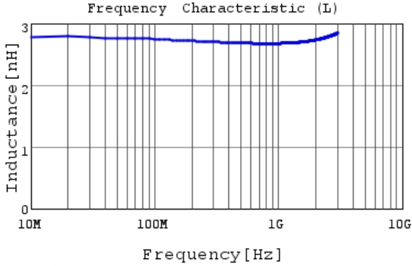
LQP15MN2N7W02 L
