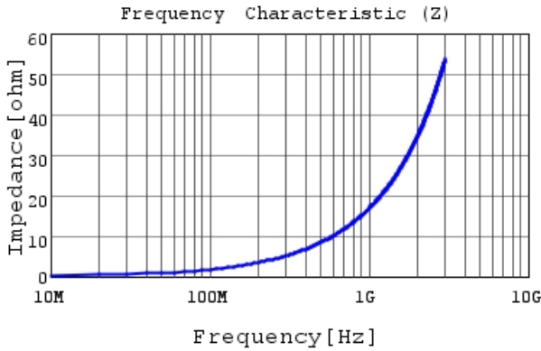
LQP15MN2N7W02 |Z|
