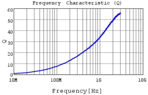
LQP15MN2N7W02 Q
