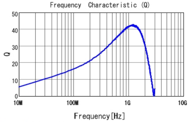
LQG15WH23NG02 Q
