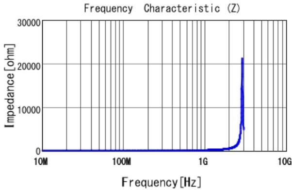
LQG15WH23NG02 |Z|
