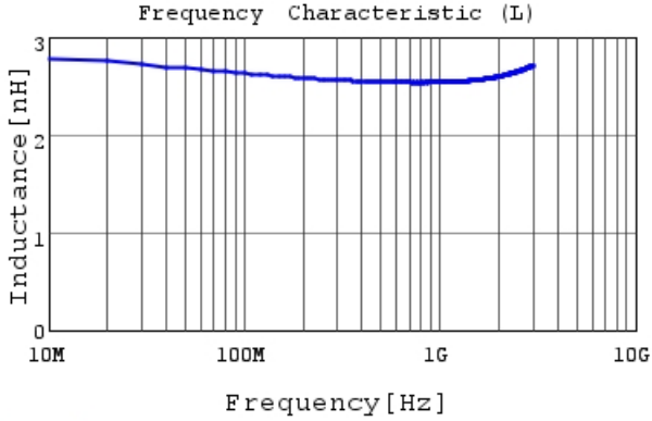
LQP03TQ2N5C02 L
