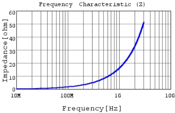
LQP03TQ2N5C02 |Z|
