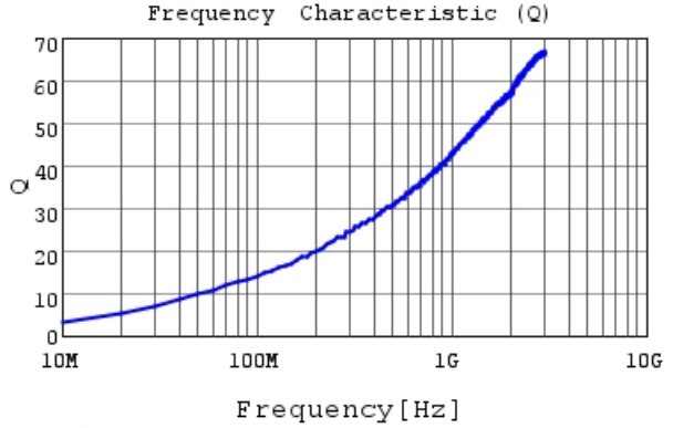
LQP03TQ2N5C02 Q
