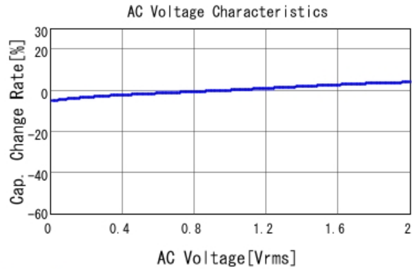
GRM32MB11C225KA01 C-AC Voltage capchange, DCOV, 2C
