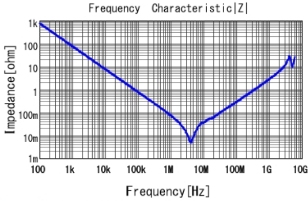
GRM32MB11C225KA01 |Z| DCOV, 20degC
