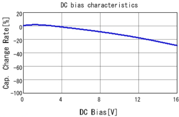
GRM32MB11C225KA01 C-DC bias capchange, 20.0degC, A
