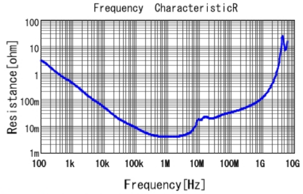
GRM32MB11C225KA01 R DCOV, 20degC
