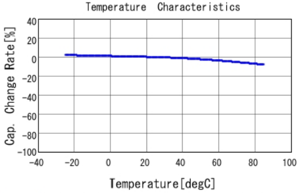
GRM32MB11C225KA01 C-Temp. capchange, DC0.0V, AC1.C
