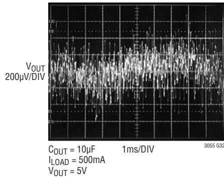
10Hz to 100kHz Output Noise C_{REF/BYP} = 10\text{nF} , C_{FF} = 0
