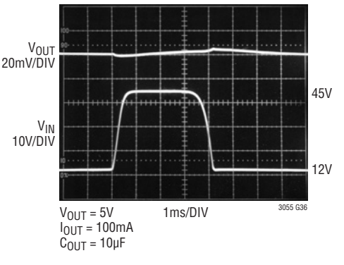
Transient Response (Load Dump)
