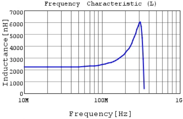
LQW21HN2R2J00 L
