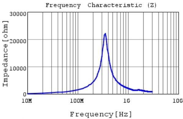
LQW21HN2R2J00 |Z|
