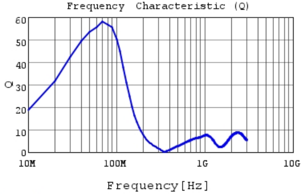
LQW21HN2R2J00 Q
