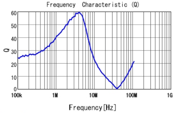
LQH5BPN3R3N38 Q
