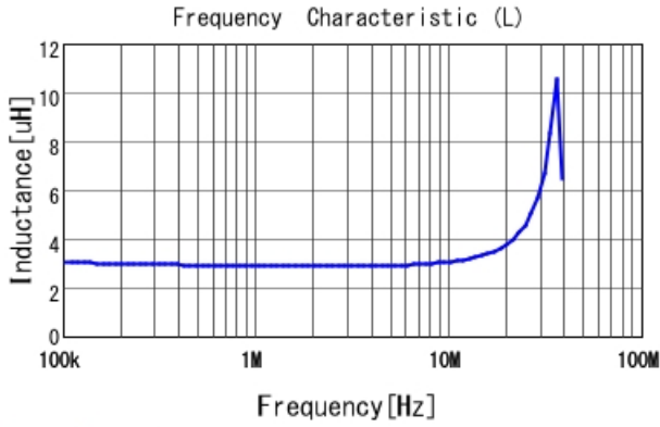
LQH5BPN3R3N38 L
