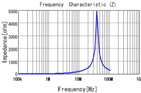
LQH5BPN3R3N38 |Z|
