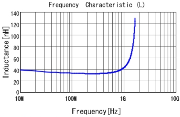
LQG15HN33NG02 L
