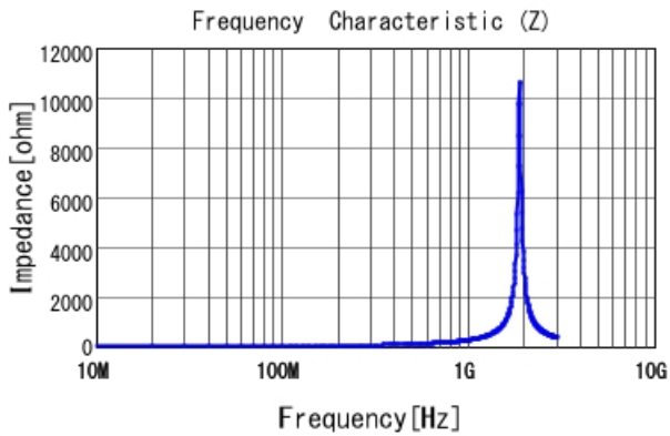
LQG15HN33NG02 |Z|
