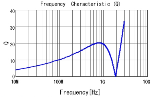
LQG15HN33NG02 Q
