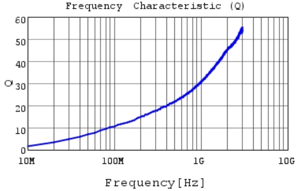
LQP02HQ3N1B02 Q
