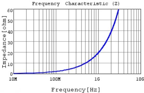
LQP02HQ3N1B02 |Z|
