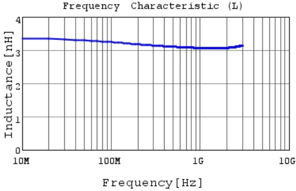
LQP02HQ3N1B02 L
