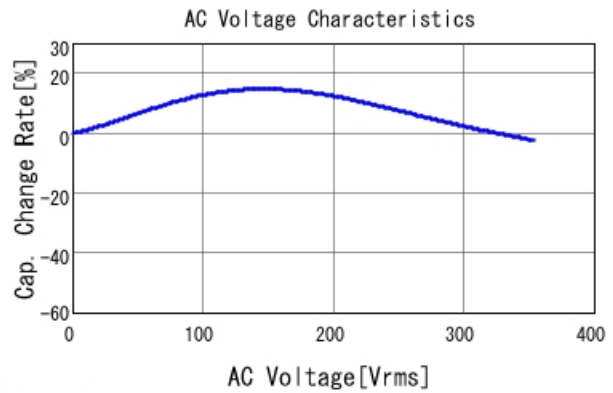
GRM31BR73A471KW01 C-AC Voltage capchange, DCOV, 25
