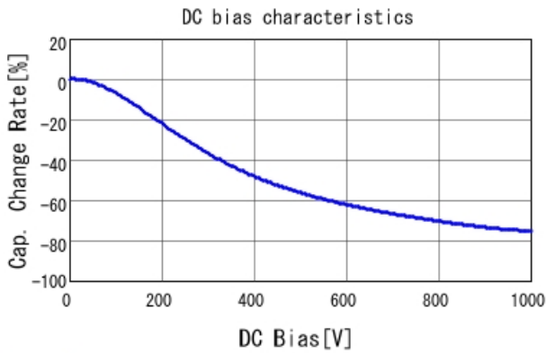
GRM31BR73A471KW01 C-DC bias capchange, 25.0degC, A
