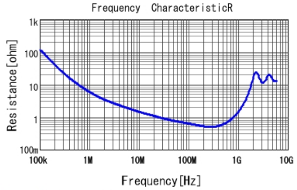
GRM31BR73A471KW01 R DCOV, 25degC
