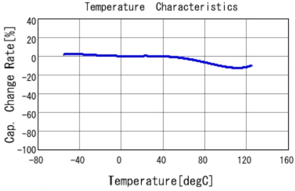
GRM31BR73A471KW01 C-Temp. capchange, DCOV, AC1Vrms
