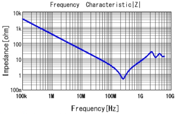
GRM31BR73A471KW01 |Z| DCOV, 25degC
