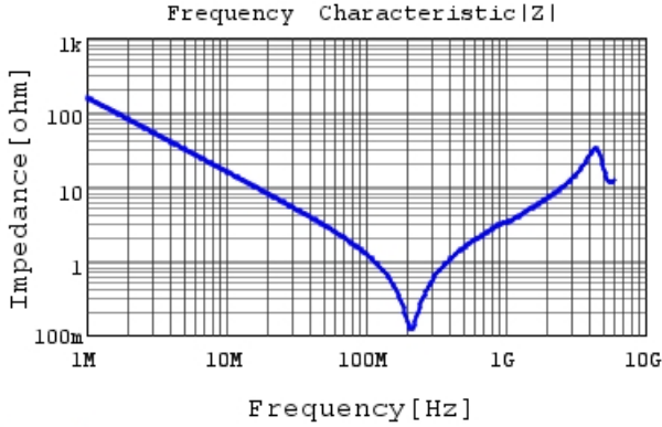
GCM2199E2A102MA05 |Z| DC0V, 20degC
