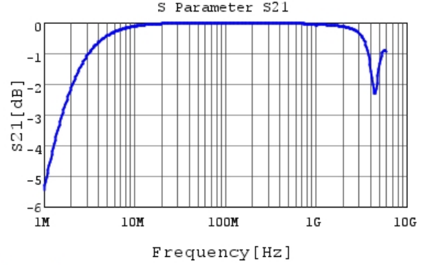
GCM2199E2A102MA05 S21 DC0V, 20degC
