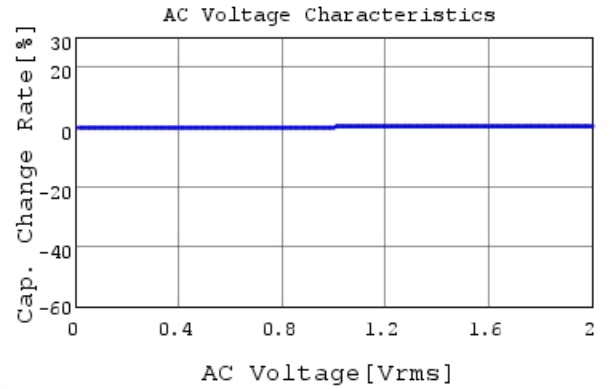
GCM2199E2A102MA05 C-AC Voltage capchange, DC
