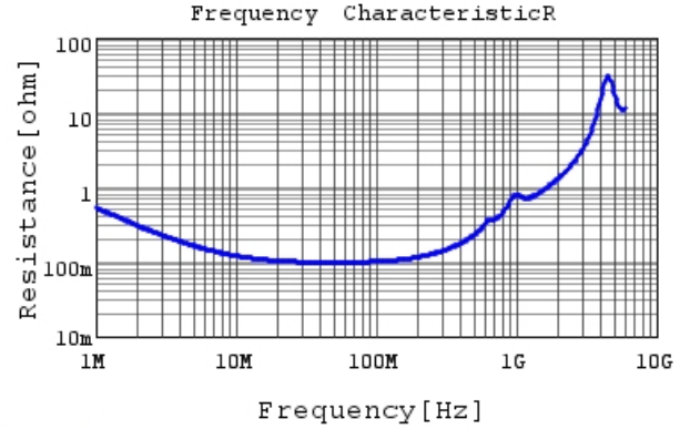
GCM2199E2A102MA05 R DC0V, 20degC
