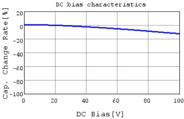
GCM2199E2A102MA05 C-DC bias capchange, 20.0c
