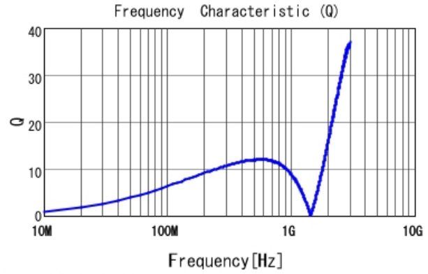
LQP03TN82NJZ2 Q
