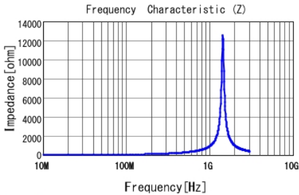
LQP03TN82NJZ2 |Z|
