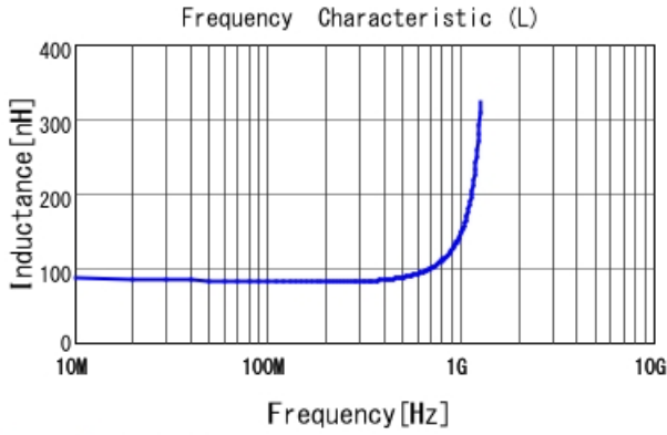
LQP03TN82NJZ2 L
