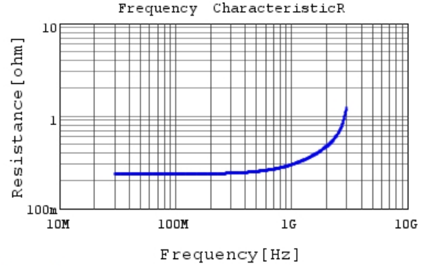
RDE5C2A220J0P1H03B R DC0V, 25degC
