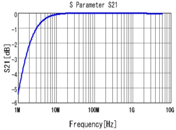
■ GRM0332C1E102JA01 S21 DCOV, 20degC
