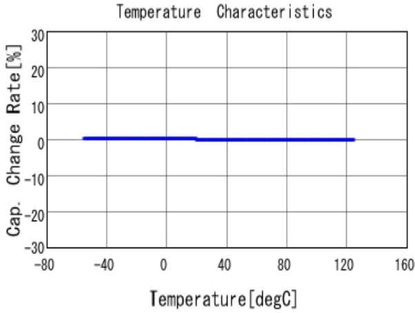
■ GRM0332C1E102JA01 C-Temp. capchange, DCOV, AC1Vrms
